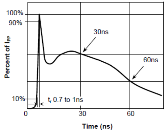
Fig.4 Pulse Waveform-ESD(IEC61000-4-2)
