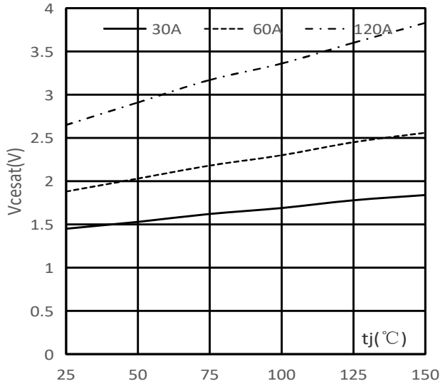
饱和压降-温度特性/ V_{cesat} as a function
