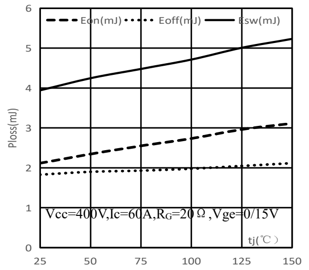
动态损耗-温度特性/Typical switching losses of t_j
