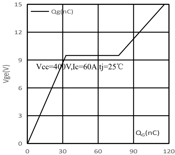
门极电量/Typical gate charge
