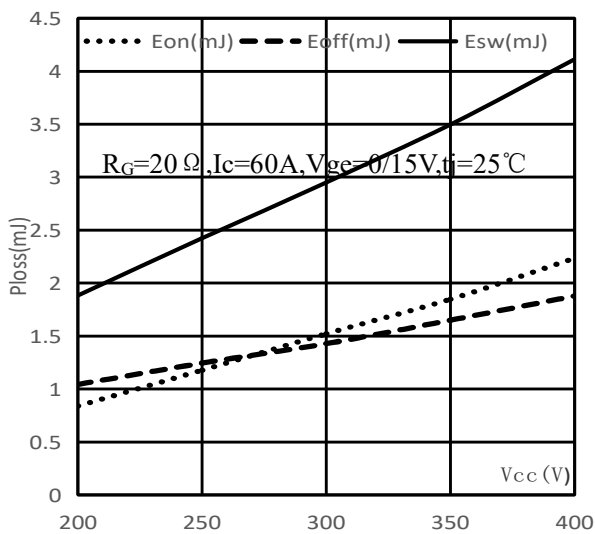
动态损耗-电压特性/Typical switching losses of V_{cc}
