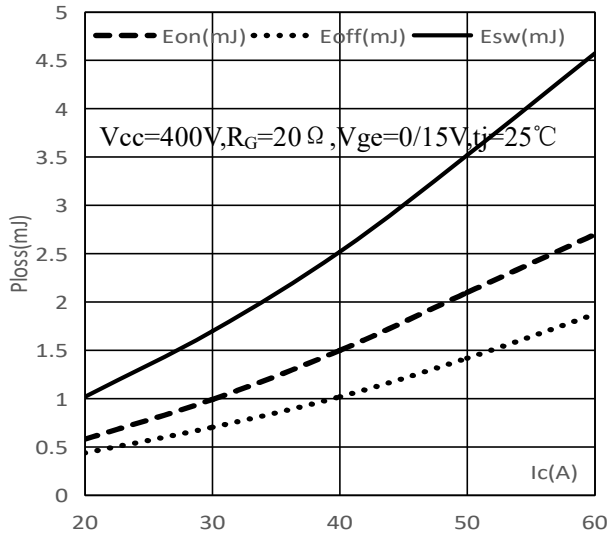
动态损耗-电流特性/Typical switching losses of I_c
