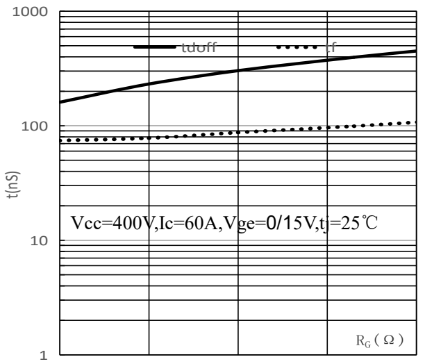
关闭时间-门极电阻特性/Typical switching times as a function of R_g
