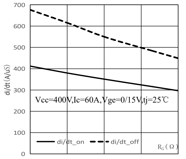
电流变化率-门极电阻特性/Typical di/dt as a function of R_g
