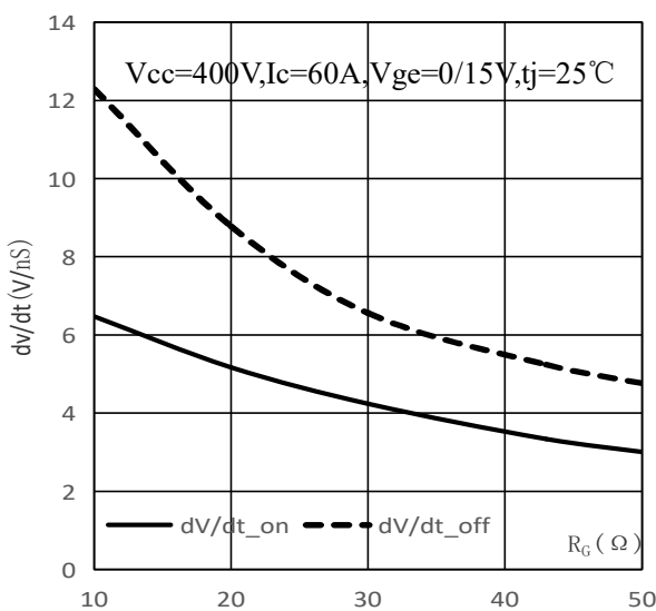
电压变化率-门极电阻特性/Typical dv/dt as a function of R_g
