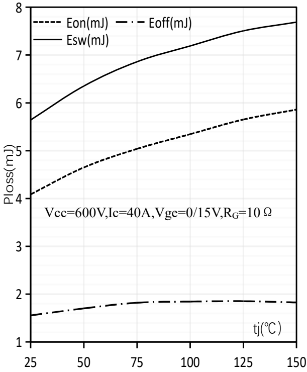
动态损耗-温度特性/Typical switching losses of t_j
