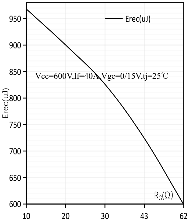
反向恢复损耗-门极电阻特性/Typical E_{REC} as a function of R_G
