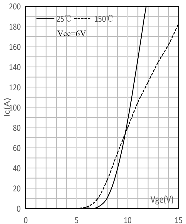
输出特性/ Typical Output Characteristic
