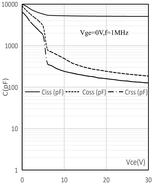
寄生电容/Capacitance as a function of Vce
