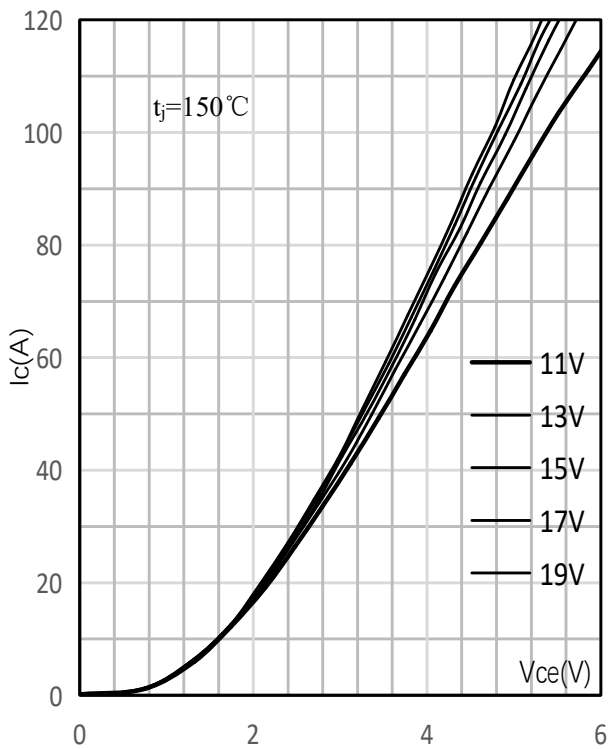
输出特性_150°C/ Typical Output Characteristic_150°C
