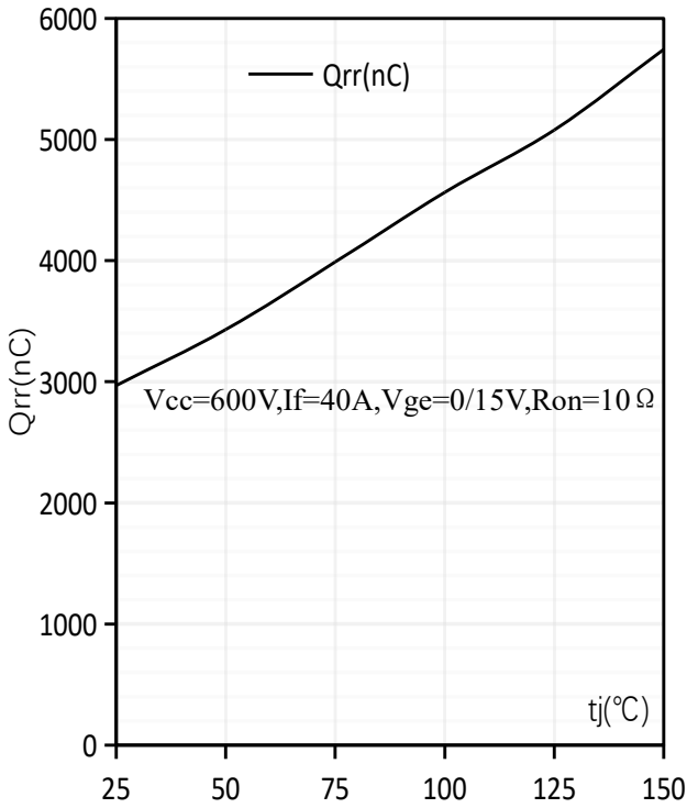
反向恢复电量-温度特性/Typical Q_{rr} as a function of t_j
