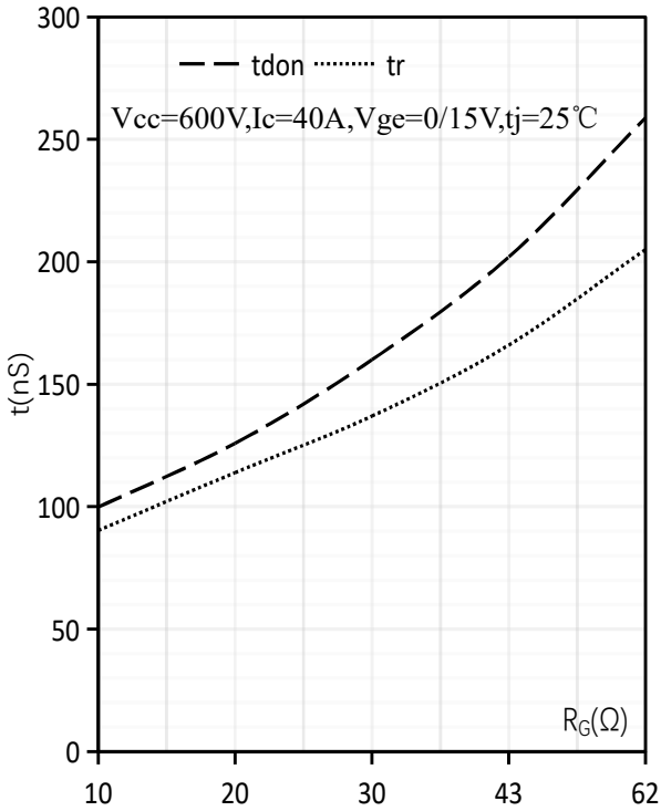
开启时间-门极电阻特性/Typical switching times as a function of R_G
