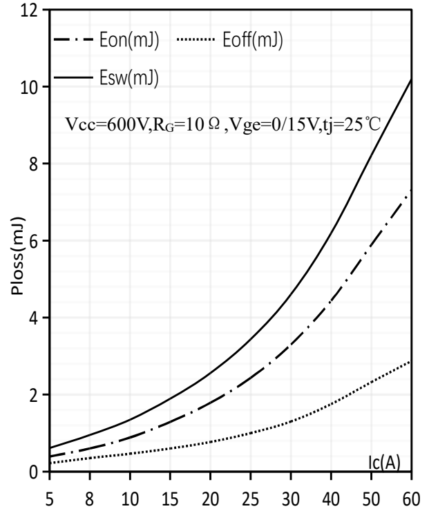
动态损耗-电流特性/Typical switching losses of I_c
