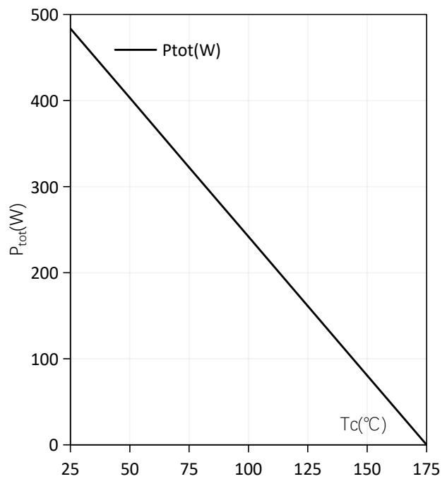
耗散功率-温度特性/P tot as a function of case Temperature
