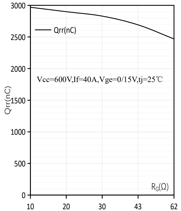
反向恢复电量-门极电阻特性/Typical Q_{rr} as a function of R_G
