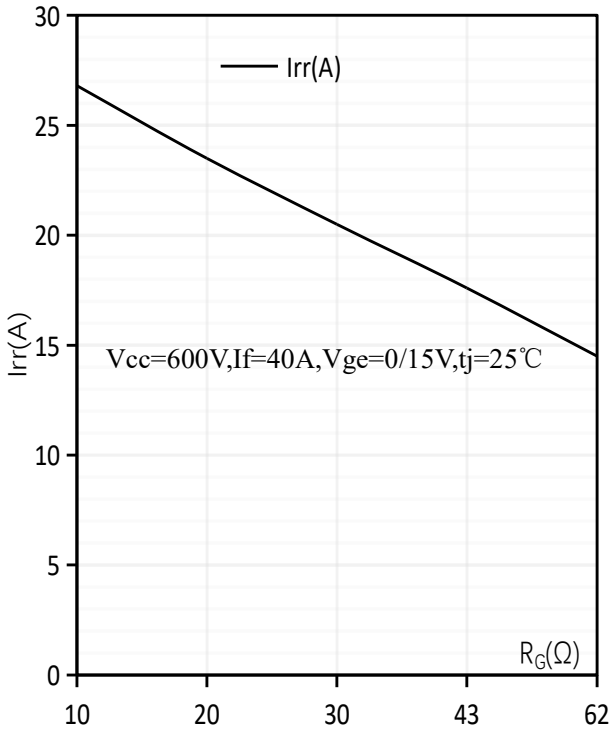
反向恢复电流峰值-门极电阻特性/Typical I_{rr} as a function of R_G
