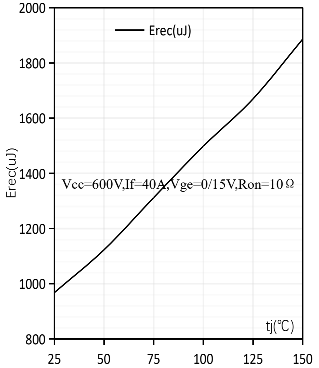
反向恢复损耗-温度特性/Typical E_{REC} as a function of t_j
