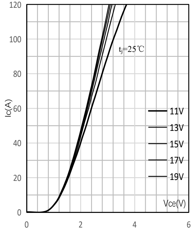
输出特性_25°C/ Typical Output Characteristic_25°C
