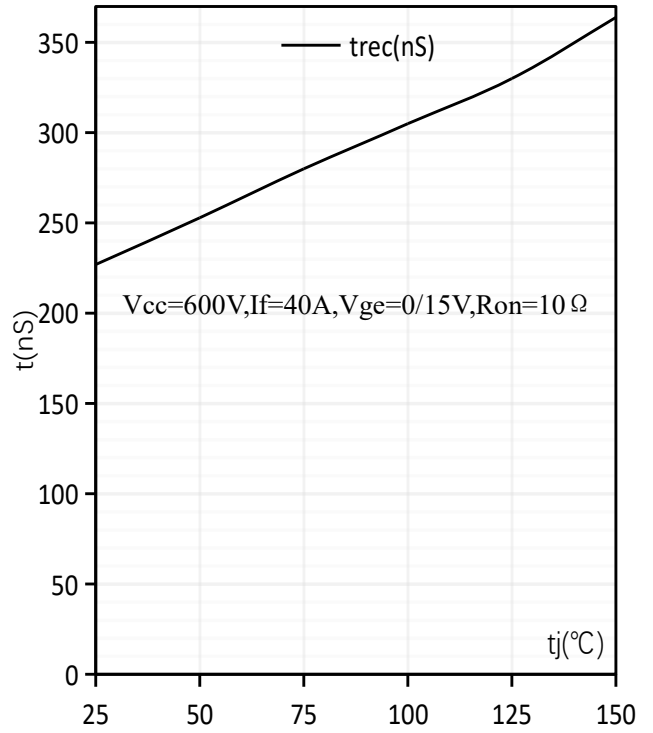
反向恢复时间-温度特性/Typical t_{rec} as a function of t_j
