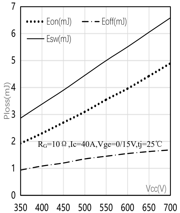
动态损耗-电压特性/Typical switching losses of V_{CC}
