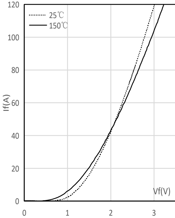
二极管压降/Typical I_F as a function of V_F
