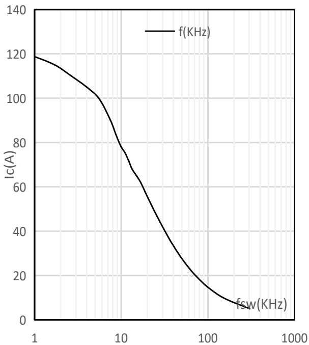
频率-电流特性/Typical fsw as a function of IC
