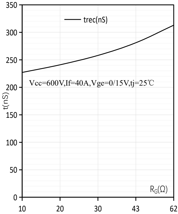
反向恢复时间-门极电阻特性/Typical t_{rec} as a function of R_G
