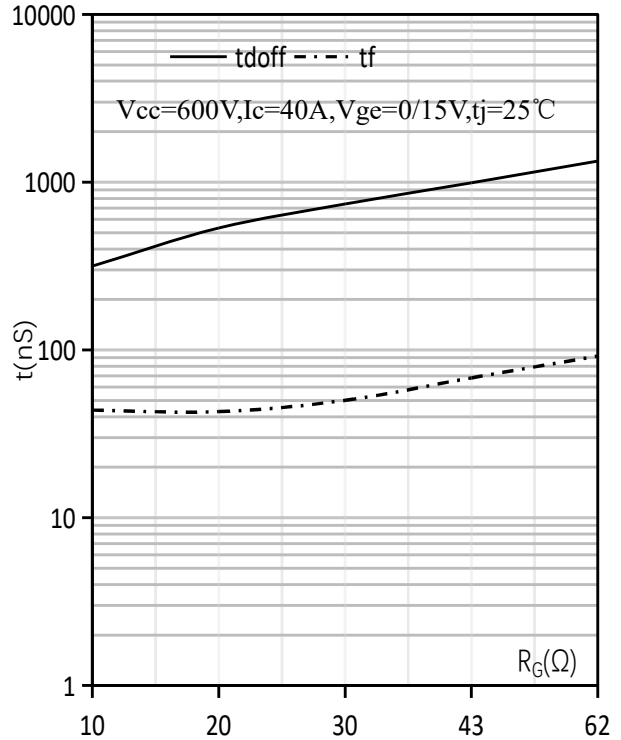
关闭时间-门极电阻特性/Typical switching times as a function of R_G
