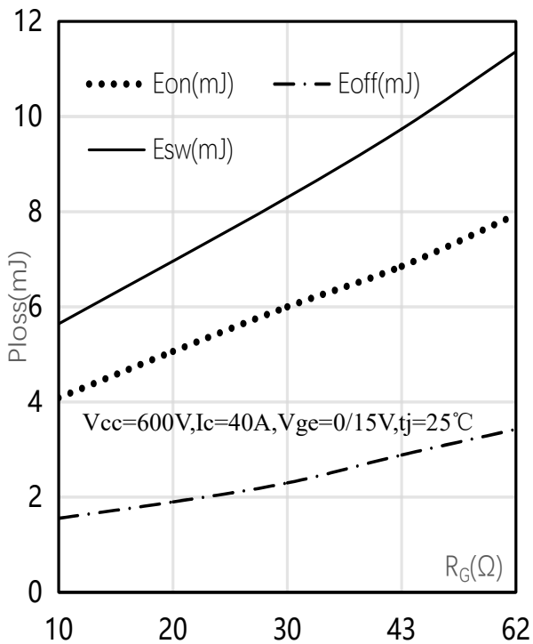
动态损耗-门极电阻特性/Typical switching losses of R_G
