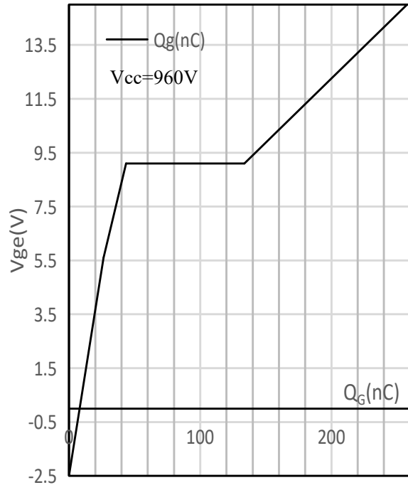
门极电量/Typical gate charge
