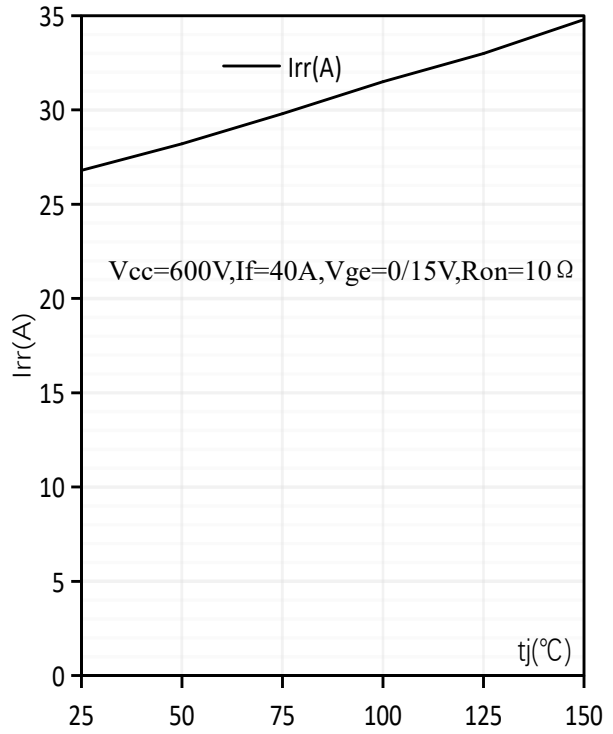
反向恢复电流峰值-温度特性/Typical I_{rr} as a function of t_j
