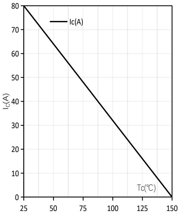
电流-底板温度特性/ I_c as a function of case temperature
